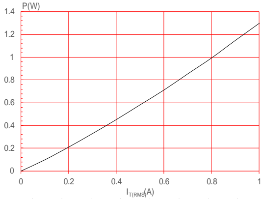
FIG.1: Min RMS
